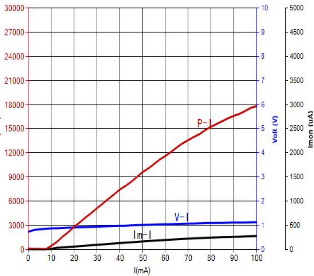
PIV Curve
